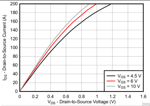
Figure 2. Saturation Characteristics
