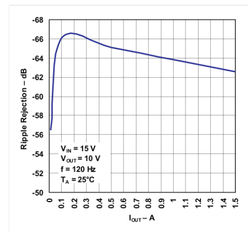
Figure 6. Ripple Rejection vs Output Current
