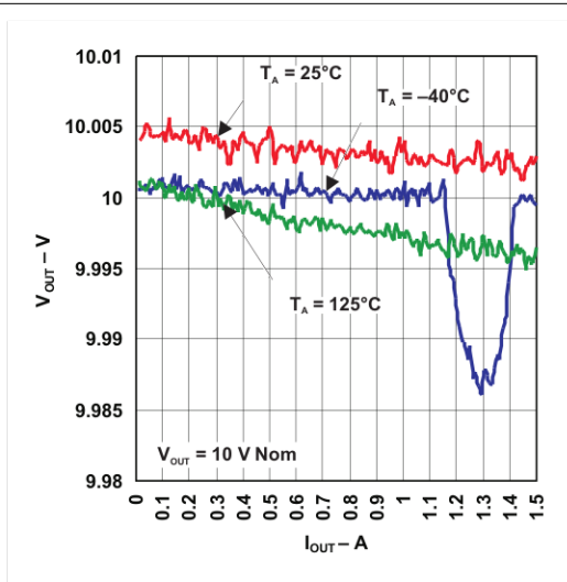
Figure 1. Load Regulation
