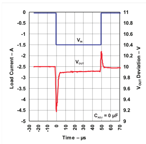
Figure 3. Load Transient Response
