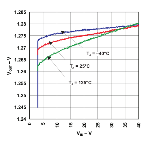
Figure 5. Line Regulation
