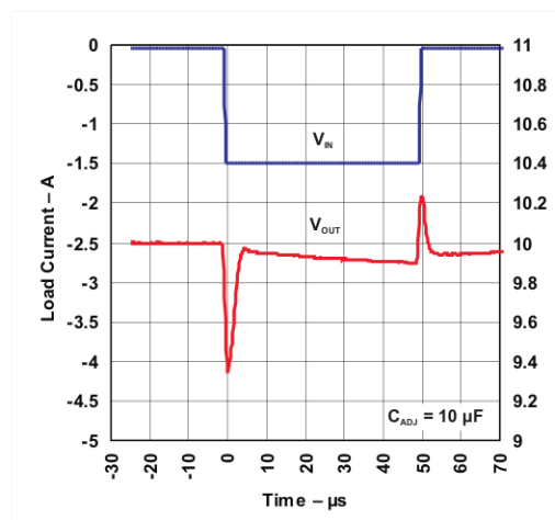
Figure 4. Load Transient Response
