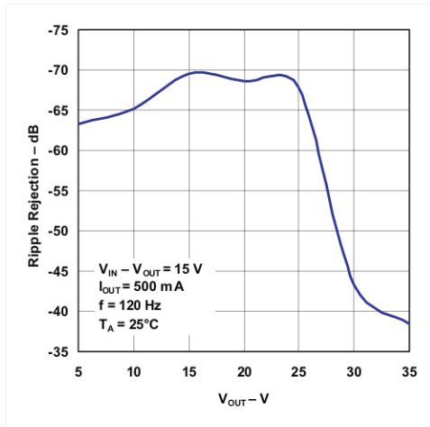
Figure 7. Ripple Rejection vs Output Voltage
