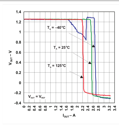
Figure 2. Load Regulation
