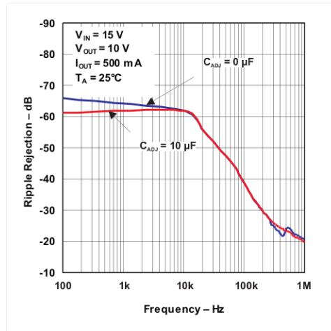
Figure 8. Ripple Rejection vs Frequency
