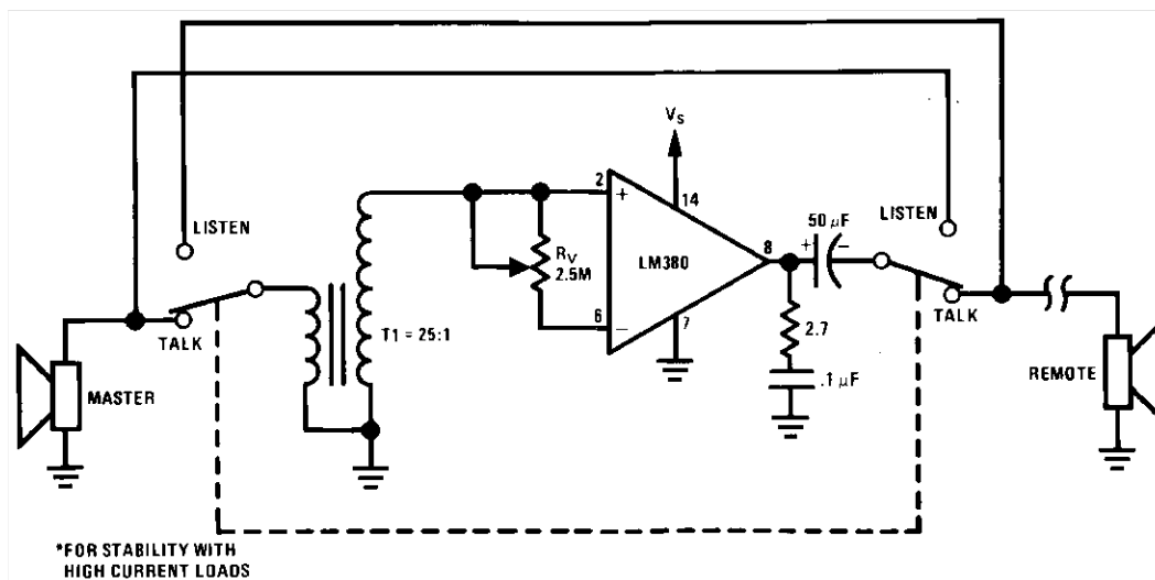
Figure 18. Intercom
