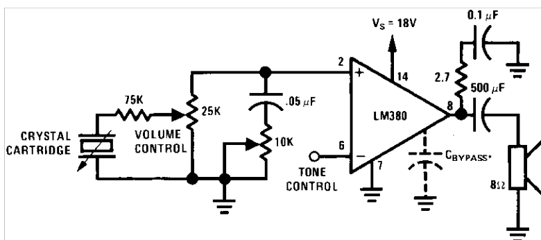
Figure 16. Phono Amplifier
