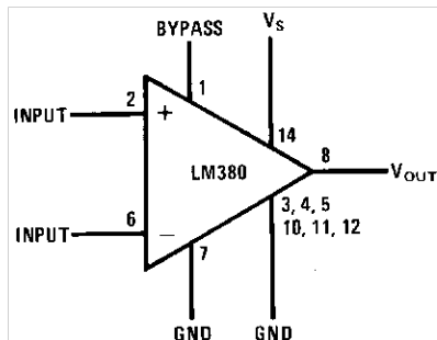
Figure 3. 14-Pin PDIP
