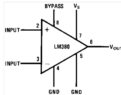
Figure 4. 8-Pin PDIP
