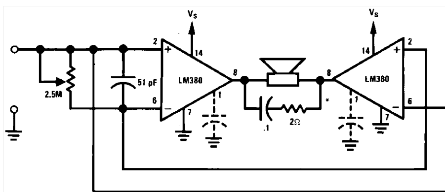
Figure 17. Bridge Amplifier
