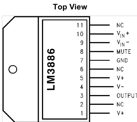
Figure 2. TO-220 and PFM Plastic Packages See Package Number NDJ0011B for Staggered Lead Non-Isolated Package or NDA0011B for Staggered Lead Isolated Package (1)
