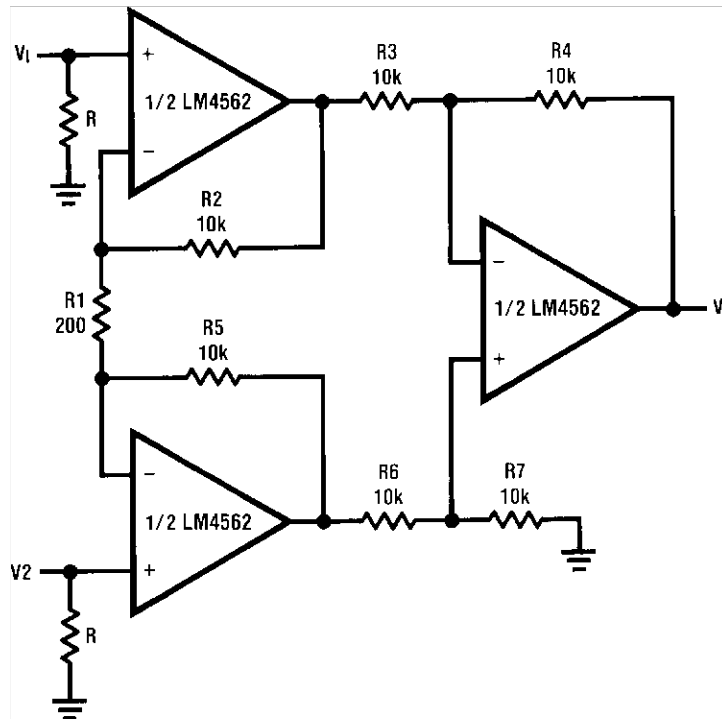
Figure 126. RIAA Preamp
