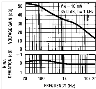
Figure 111. RIAA Preamp Voltage Gain, RIAA Deviation vs Frequency
