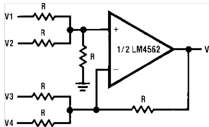
Figure 117. Adder/Subtractor
