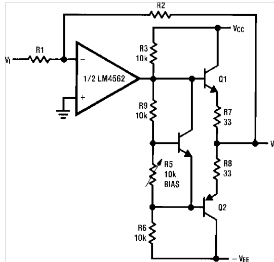
Figure 124. Line Driver
