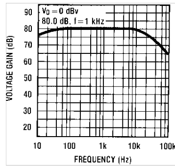
Figure 112. Flat Amp Voltage Gain vs Frequency
