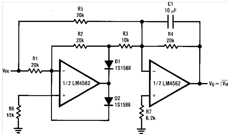
Figure 122. AC/DC Converter
