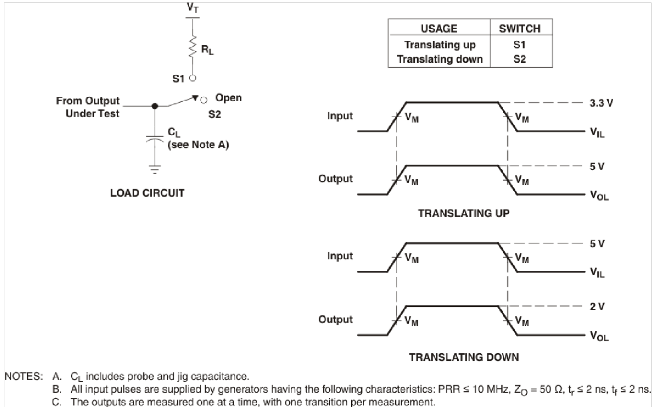
Figure 7-1. Load Circuit for Outputs
