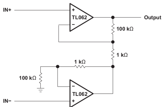
Figure 28. Instrumentation Amplifier
