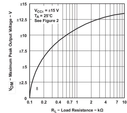
Figure 6-45. Maximum Peak Output Voltage vs Load Resistance
