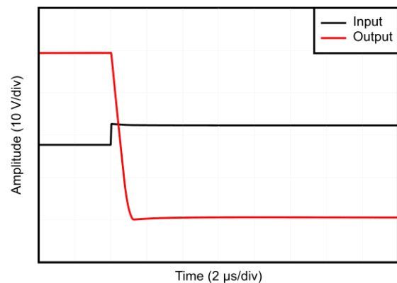
Figure 6-28. No Phase Reversal
