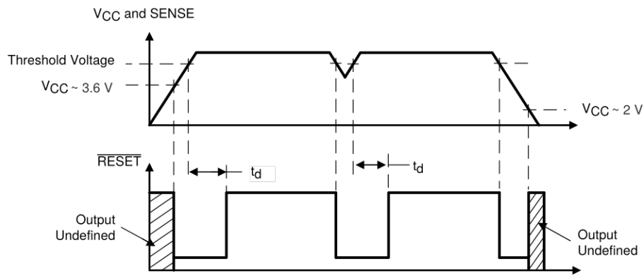
Figure 1. Timing Diagram
