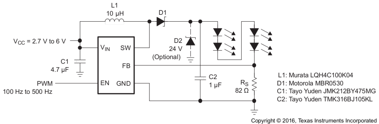
Figure 21. White LED Supply With Adjustable Brightness Control
