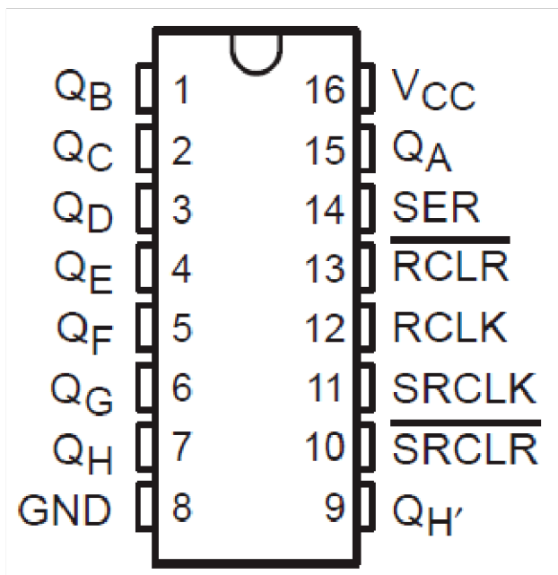
Pin Functions
