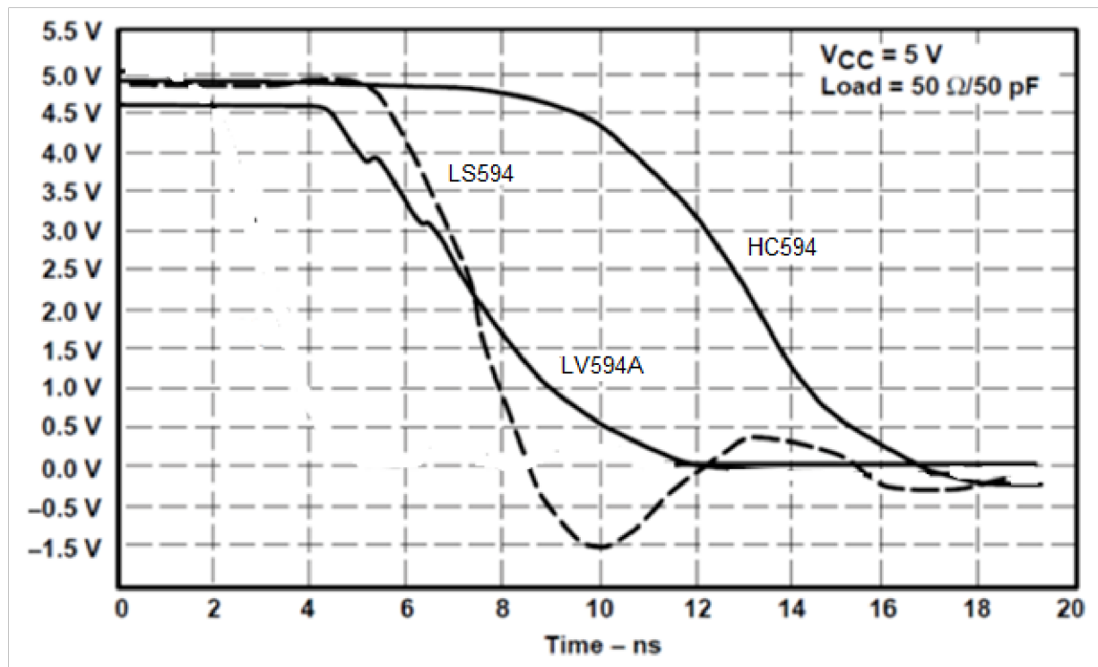
Figure 7. Switching Characteristics Comparison
