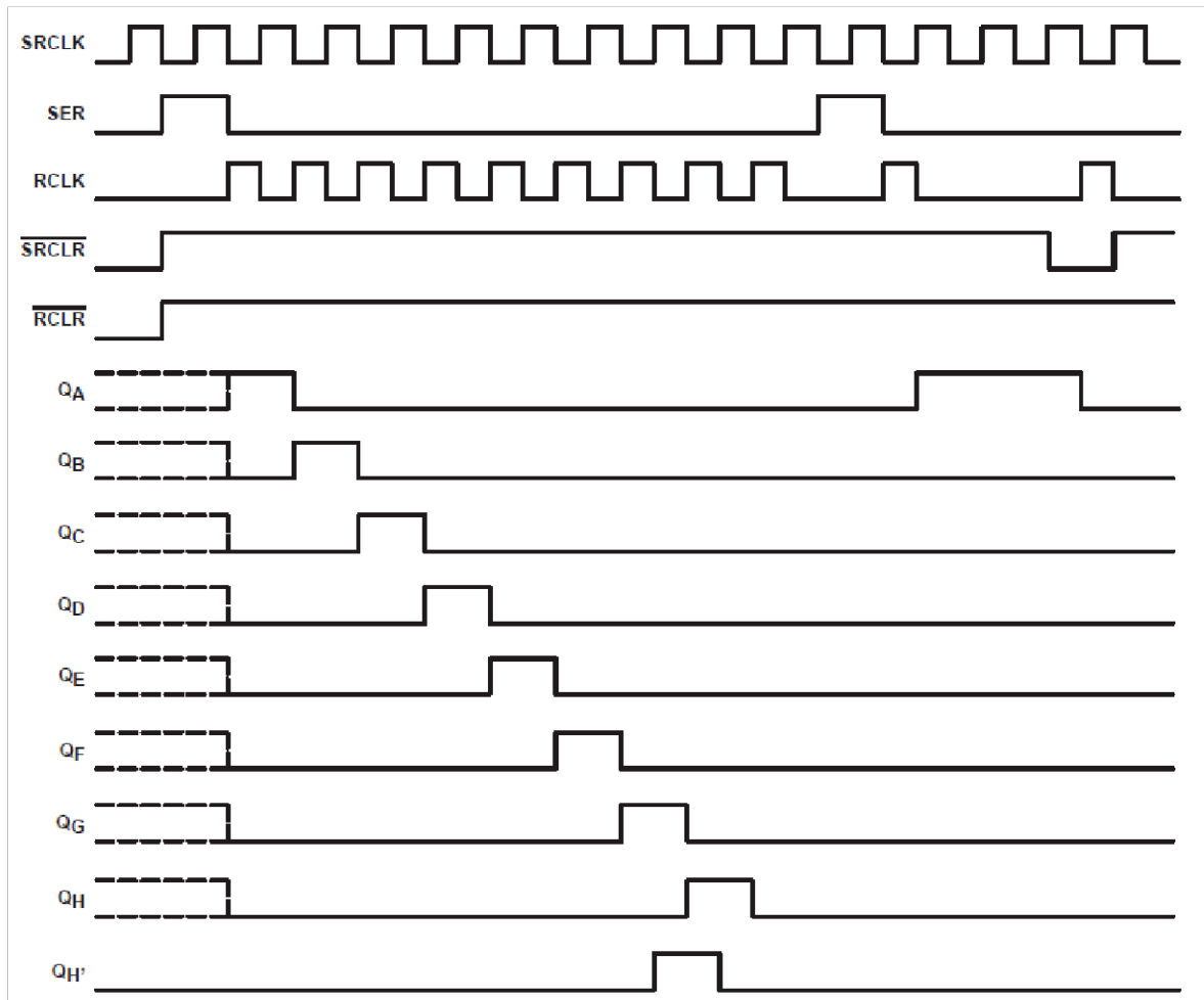
Figure 1. Timing Diagram
