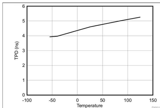
Figure 2. TPD vs. Temperature at 3.3 V
