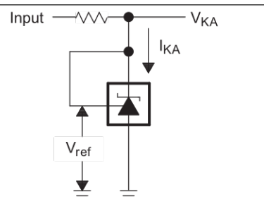
Figure 22. Test Circuit for V_{KA} = V_{ref}
