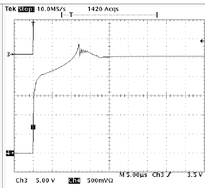
Figure 34. ATL43x Start-up Response I_{KA} = 1 mA
