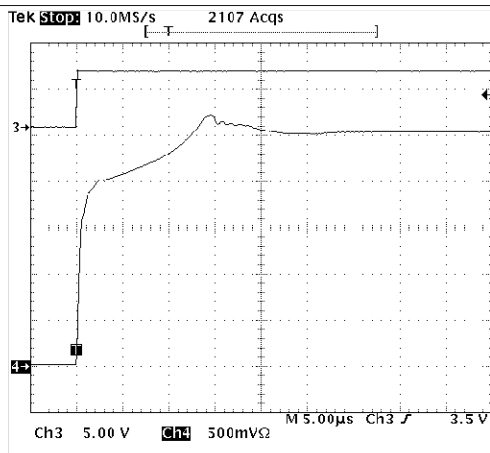
I_{KA} = 100 \mu A Figure 28 used for this measurement.
