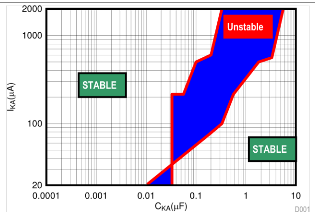
ESR < 20 mΩ Figure 27 used to verify stability.
