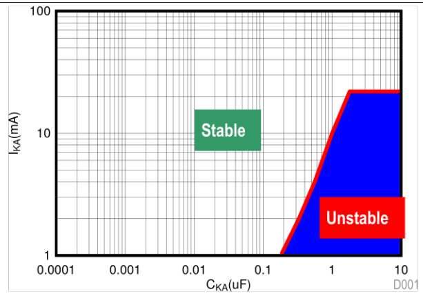
ESR < 20 mΩ Figure 27 used to verify stability.
