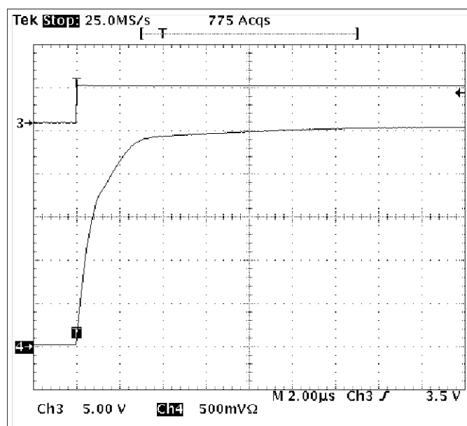
Figure 33. ATL43x Start-up Response I_{KA} = 50 \mu A
