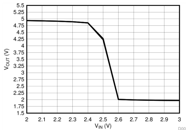
Figure 31. Open Loop (Comparator Mode) V_{OUT} vs V_{IN}
