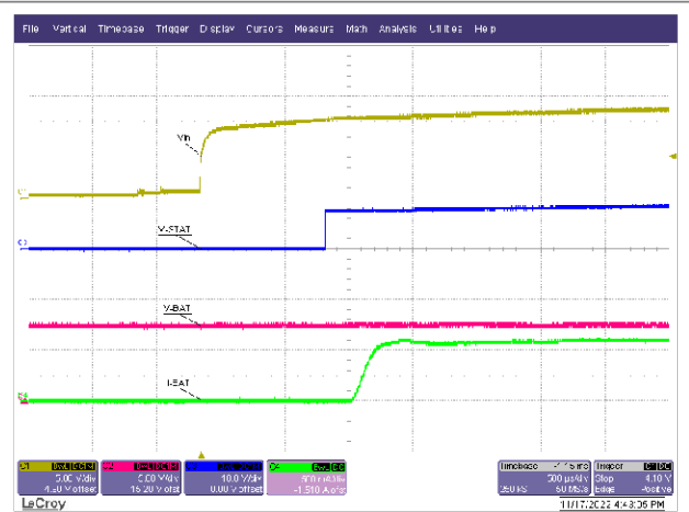
Figure 10-16. Charge Profile with Battery Simulator - STAT
