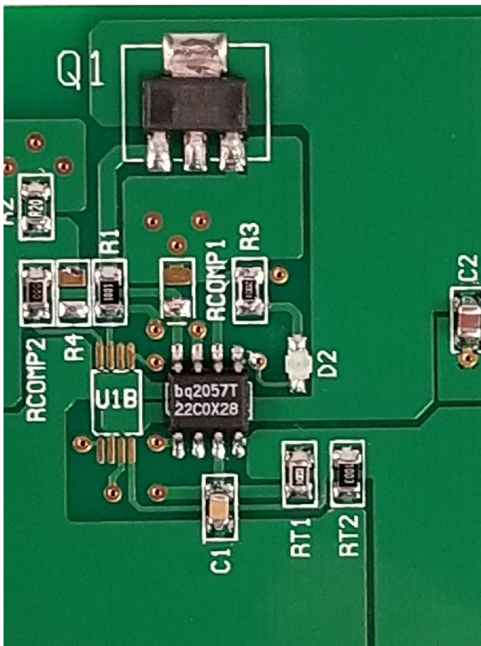
Figure 12-1. Layout Example
