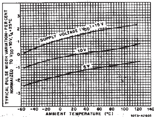
Fig. 10 - Typical pulse-width variation as a function of temperature ( R_x=100 K\Omega , C_x=0.1 \mu F ).
