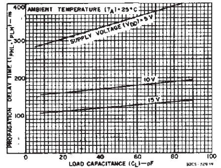
Fig. 8—Typical propagation delay time as a function of load capacitance (Astable, \bar{A} stable to Q, \bar{Q} ).
