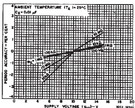
Fig. 12—Typical astable oscillator or Q, Q̄ period accuracy vs. supply voltage.
