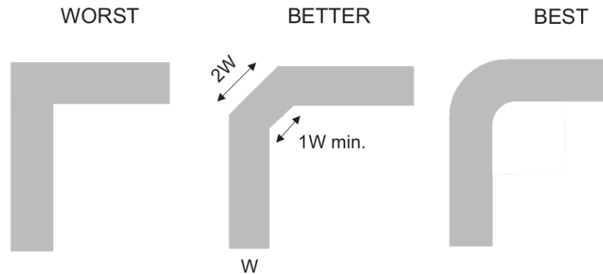
Figure 31. Trace Example
