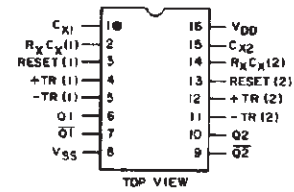
TERMINALS 1, 8, 15 ARE ELECTRICALLY CONNECTED INTERNALLY 92CS-24846R1 TERMINAL ASSIGNMENT
