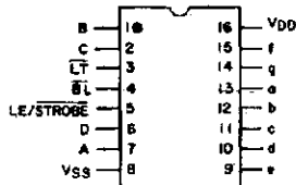
TOP VIEW 92CS-25084B CD4511B TERMINAL ASSIGNMENT
