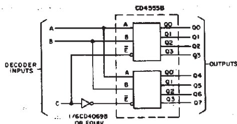
Fig. 20 - 1-of-8 decoder using CD4555B.
