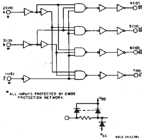
Fig. 5 — CD4555B logic diagram (1 of 2 identical circuits).
