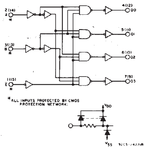
Fig. 6 — CD4556B logic diagram (1 of 2 identical circuits).
