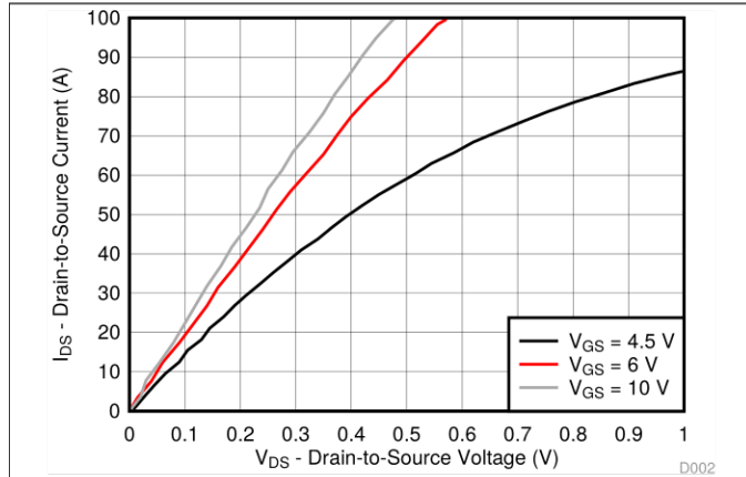
Figure 2. Saturation Characteristics
