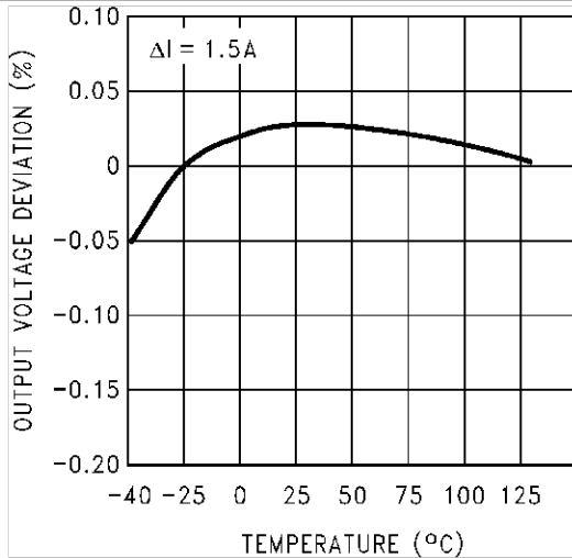
Figure 3. Load Regulation
