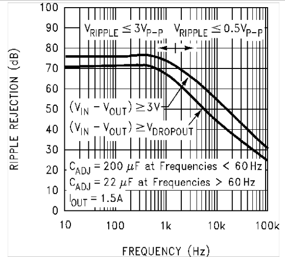
Figure 4. LM1084-ADJ Ripple Rejection
