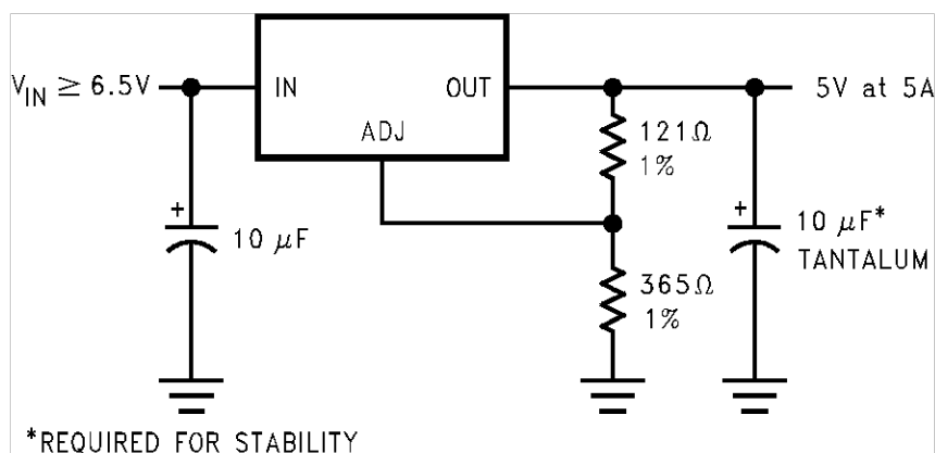
Figure 17. Adjustable @ 5 V
