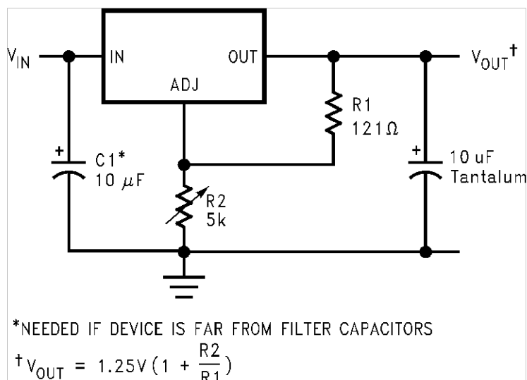
Figure 16. 1.2-V to 15-V Adjustable Regulator
