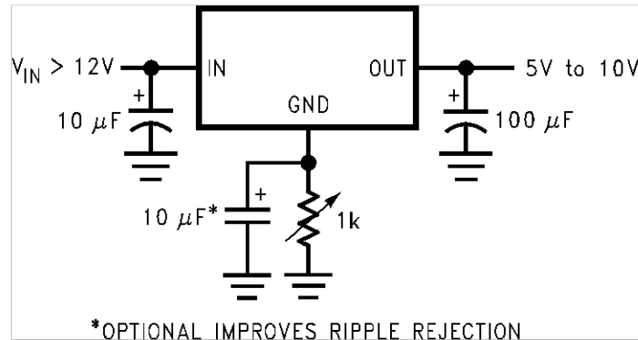
Figure 20. Adjustable Fixed Regulator
