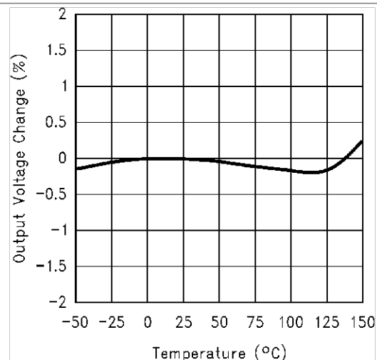
Figure 6. Temperature Stability
