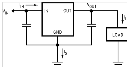
Figure 29. Power Dissipation Diagram
