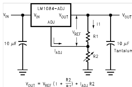
Figure 14. Basic Adjustable Regulator
