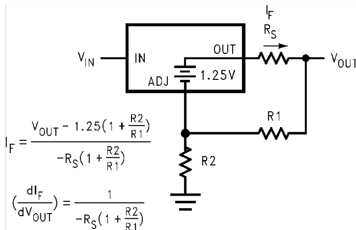
Figure 19. Battery Charger
