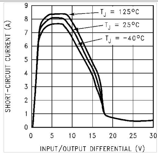
Figure 2. Short-Circuit Current
