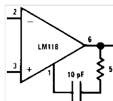
Figure 41. Overcompensation
