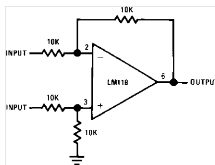
Figure 45. Differential Amplifier
