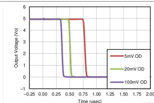
Figure 8-3. Response Time for Various Overdrives (Negative Transition)
