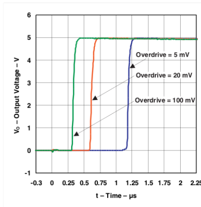
Figure 6-5. Response Time for Various Overdrives Positive Transition
