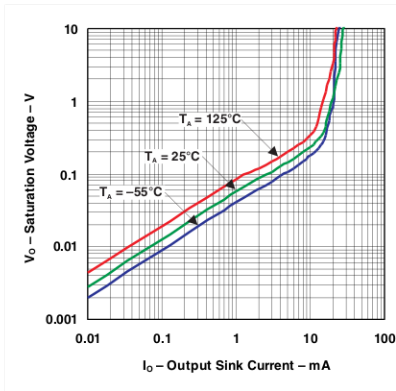
Figure 6-3. Output Saturation Voltage
