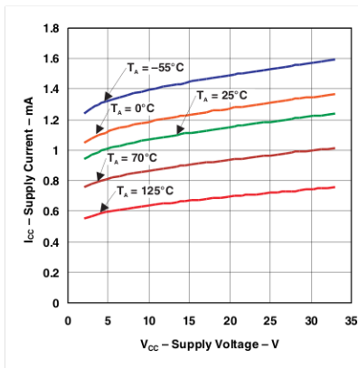
Figure 6-1. Supply Current vs Supply Voltage
