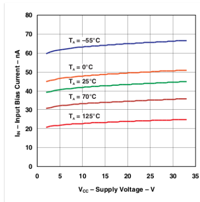
Figure 6-2. Input Bias Current vs Supply Voltage
