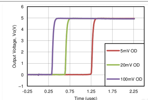
Figure 8-2. Response Time for Various Overdrives (Positive Transition)
