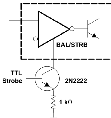
Figure 17. Offset Balancing
