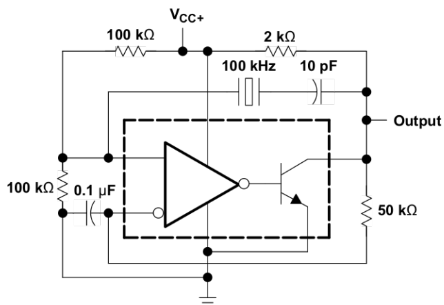
Figure 21. 100-kHz Crystal Oscillator
