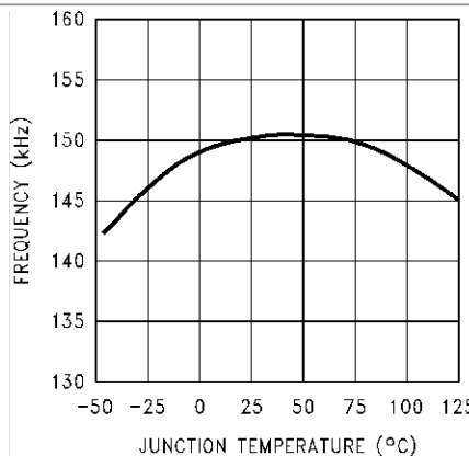
Figure 12. Switching Frequency
