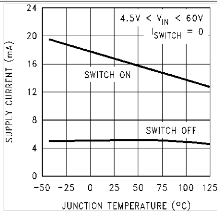
Figure 7. Quiescent Current
