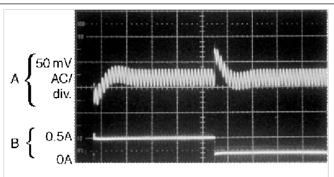
Load transient response for continuous mode V_{IN} = 20\text{ V} , V_{OUT} = 5\text{ V} , I_{LOAD} = 200\text{ mA to }500\text{ mA} L = 100\ \mu\text{H} , C_{OUT} = 120\ \mu\text{F} , C_{OUT}\text{ ESR} = 140\ \text{m}\Omega A: Output voltage, 50 mV/div. (AC) B: 200-mA to 500-mA load pulse
