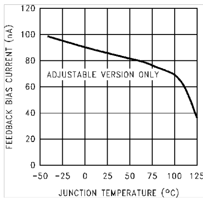
Figure 7-11. Feedback Pin Bias Current
