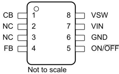
Figure 6-1. D or P Package 8-Pin SOIC or PDIP Top View
