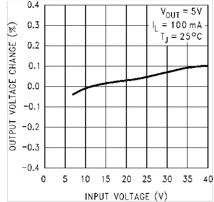
Figure 7-2. Line Regulation
