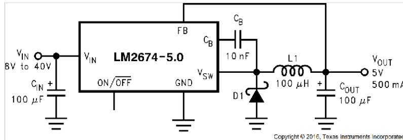
Figure 9-9. Typical Application
