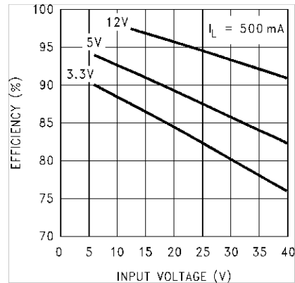
Figure 7-3. Efficiency
