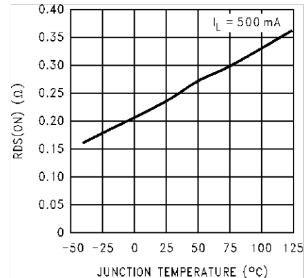
Figure 7-4. Drain-to-Source Resistance
