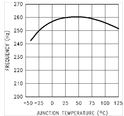
Figure 7-10. Switching Frequency
