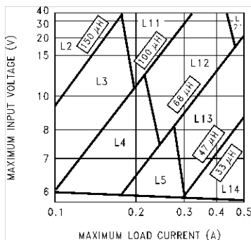
Figure 9-10. LM2674, 3.3-V Version
