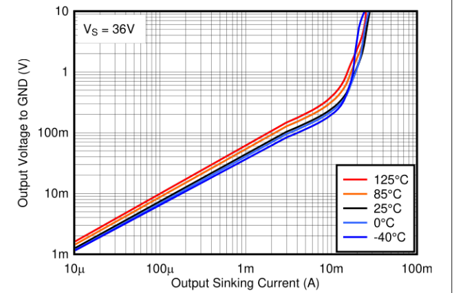
Figure 6-27. Output Low Voltage vs. Output Sinking Current at 36V
