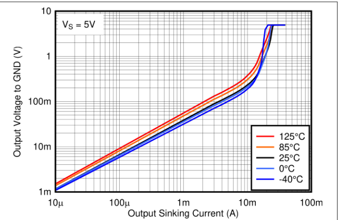
Figure 6-25. Output Low Voltage vs. Output Sinking Current at 5V
