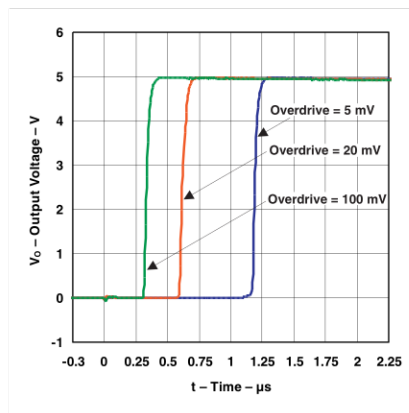
Figure 6-5. Response Time for Various Overdrives Positive Transition
