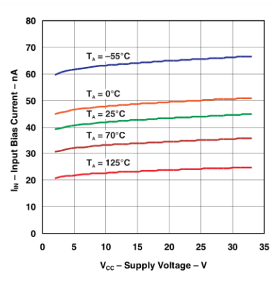
Figure 6-2. Input Bias Current vs Supply Voltage
