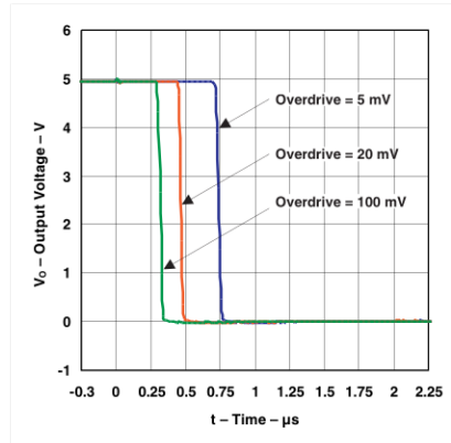
Figure 6-4. Response Time for Various Overdrives Negative Transition
