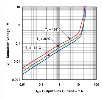
Figure 6-3. Output Saturation Voltage
