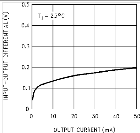
Figure 3. Dropout Voltage
