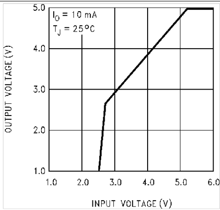
Figure 19. 5-V LM2936 Low Voltage Behavior
