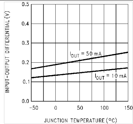
Figure 2. Dropout Voltage
