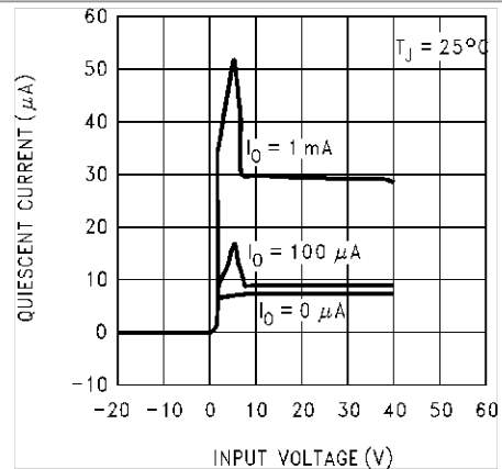
Figure 4. Quiescent Current
