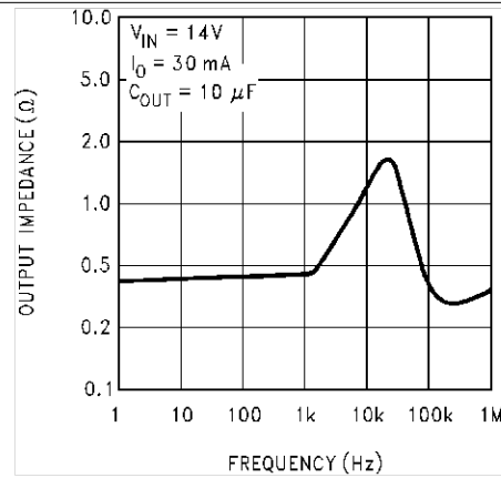
Figure 20. 5-V LM2936 Output Impedance
