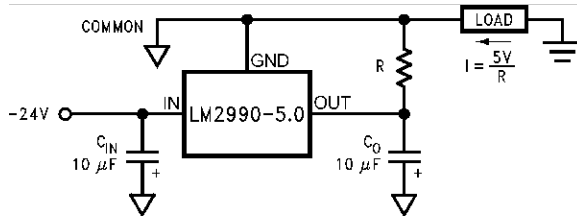
Figure 24. Fixed Current Sink
