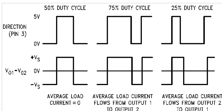
Figure 11. Locked Anti-Phase PWM Control
