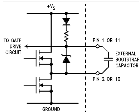
Figure 15. Bootstrap Circuitry
