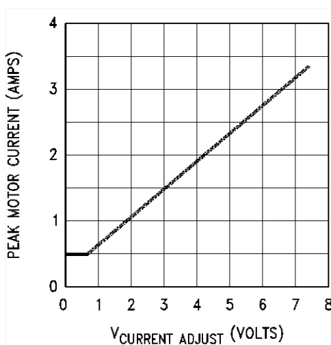
Figure 19. Peak Motor Current vs Adjustment Voltage
