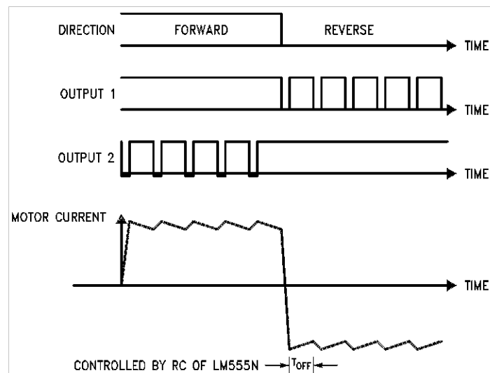
Figure 17. Switching Waveforms
