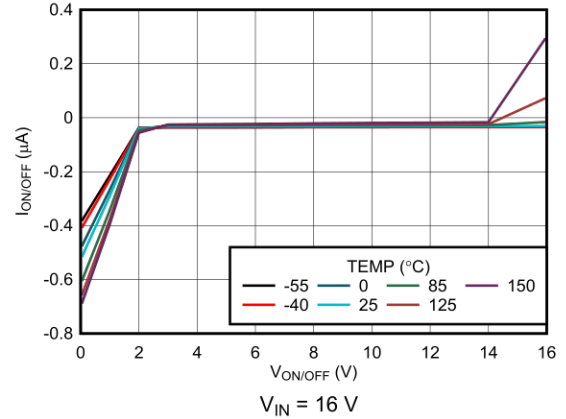
Figure 5-38. ON/OFF Pin Current versus V_{ON/OFF} (New Chip)
