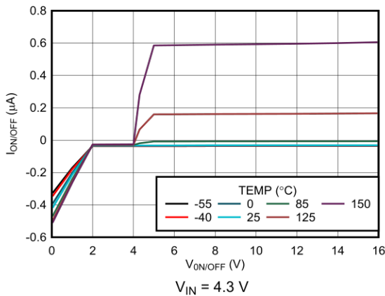
Figure 5-39. ON/OFF Pin Current versus V_{ON/OFF} (New Chip)
