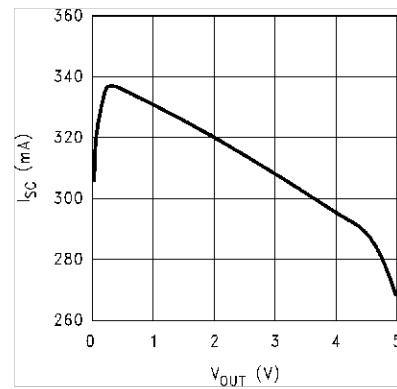
Figure 5-34. Instantaneous Short Circuit Current versus Output Voltage (Legacy chip)
