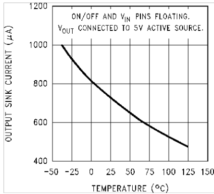
Figure 5-43. Output Reverse Leakage versus Temperature (Legacy chip)
