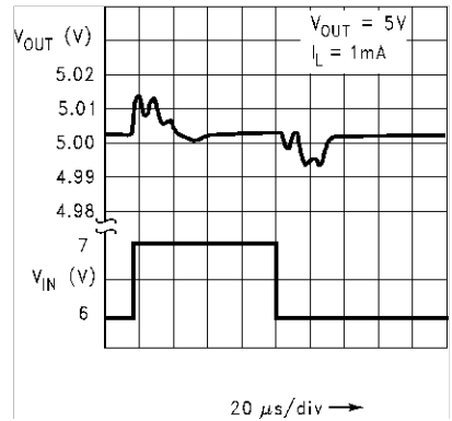
Figure 7-6. Line Transient Response (Legacy chip)
