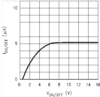
Figure 5-37. ON/OFF Pin Current versus V_{ON/OFF} (Legacy chip)
