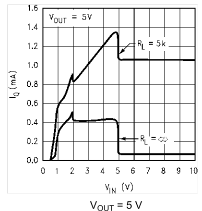
Figure 5-17. Input Current versus VIN (Legacy Chip)
