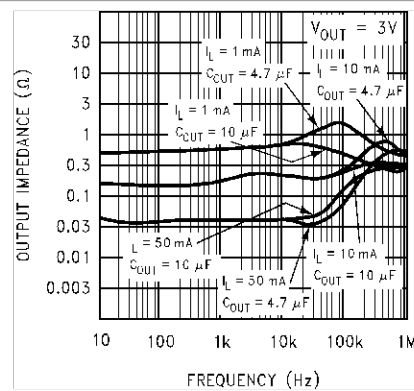
Figure 5-36. Output Impedance versus Frequency (Legacy chip)
