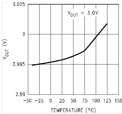
Figure 5-1. Output Voltage versus Temperature (Legacy Chip)
