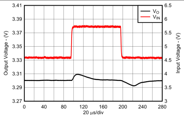
Figure 8-14. Line Transient Response for New Chip
