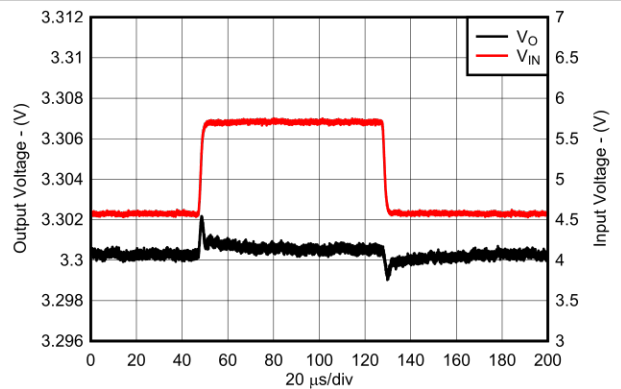
Figure 8-12. Line Transient Response for New Chip
