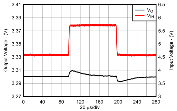
Figure 8-10. Line Transient Response for New Chip
