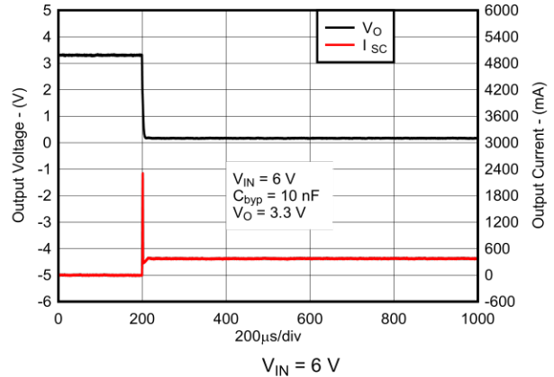
Figure 6-10. Short-Circuit Current vs Time for New Chip
