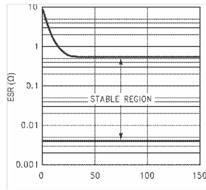
Figure 6-38. 2.2- \mu\text{F} , 3.3- \mu\text{F} Stable ESR Range for Output Voltage \geq 2.5\text{ V} for Legacy Chip
