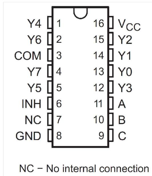
Figure 4-1. SN74HC4851 PW Package, 16-Pin TSSOP (Top View)
