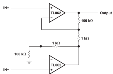
Figure 9-10. Instrumentation Amplifier
