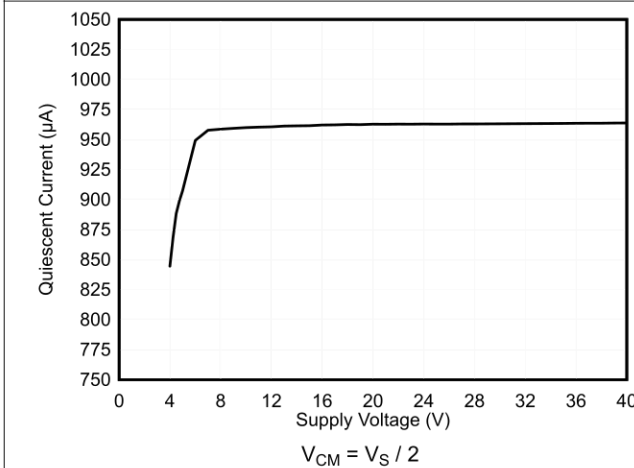
Figure 6-21. Quiescent Current vs Supply Voltage
