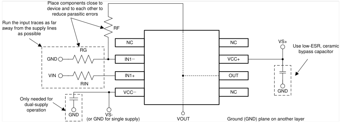
Figure 9-10. Operational Amplifier Board Layout for Noninverting Configuration
