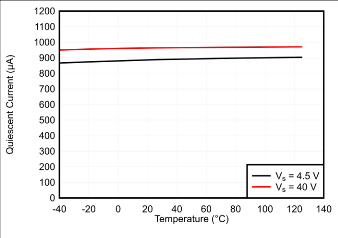
Figure 6-22. Quiescent Current vs Temperature
