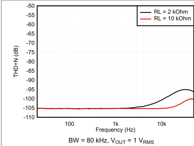
Figure 6-19. THD+N Ratio vs Frequency
