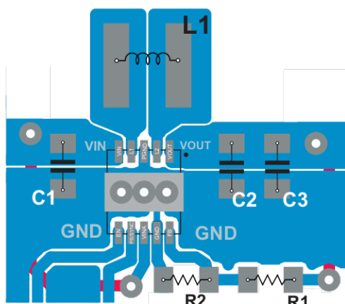
Figure 20. Layout Recommendation
