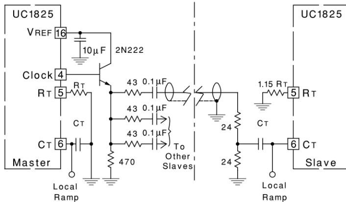
Generalized Synchronization
