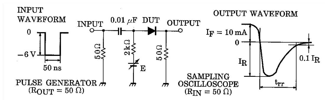
Fig. 1 Reverse Recovery Time ( t_{rr} ) Test Circuit
