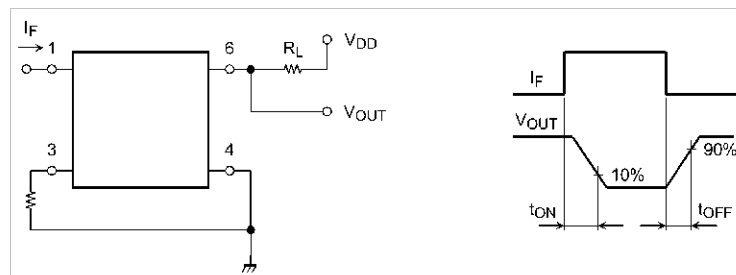
Fig. 12.1 Switching Time Test Circuit
