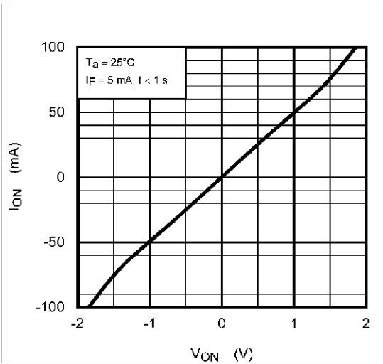
Fig. 13.1.4 I ON - V ON
