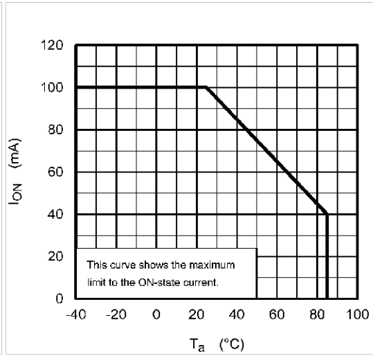
Fig. 13.1.2 I ON - T a
