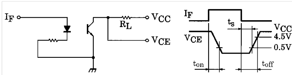
Fig. 10.1 Switching Time Test Circuit
