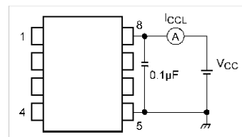
Fig. 13.1.6 I_{CCL} Test Circuit
