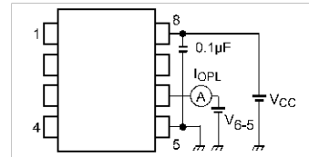
Fig. 13.1.2 I_{OPL} Test Circuit
