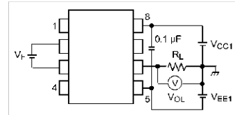
Fig. 13.1.4 V_{OL} Test Circuit
