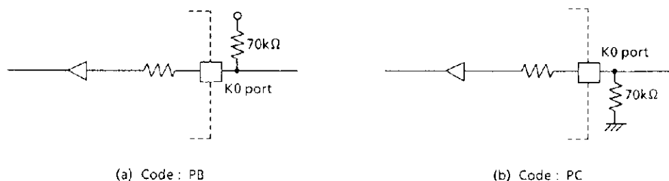
Figure 4. I/O code and external circuitry
