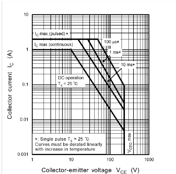
Fig. 7.7 Safe Operating Area (Guaranteed Maximum)
