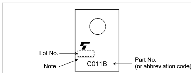
Fig. 6.1 Marking
