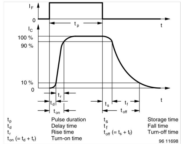
Fig. 3 - Switching Times
