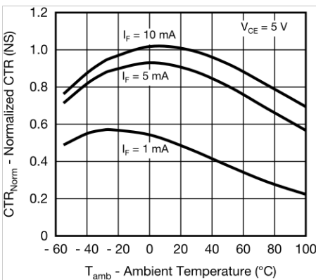
Fig. 8 - Normalized CTR (NS) vs. Ambient Temperature
