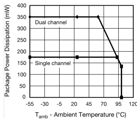
Fig. 13 - Power Dissipation vs. Ambient Temperature
