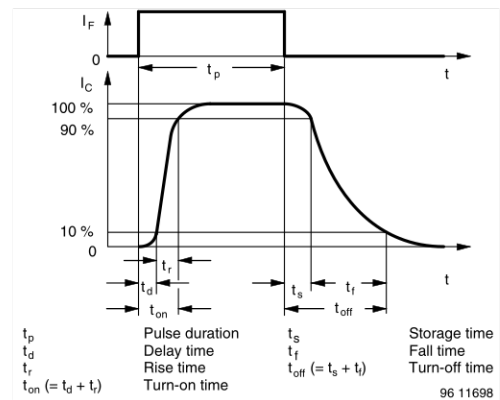
Fig. 3 - Switching Times
