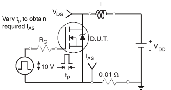
Fig. 12a - Unclamped Inductive Test Circuit
