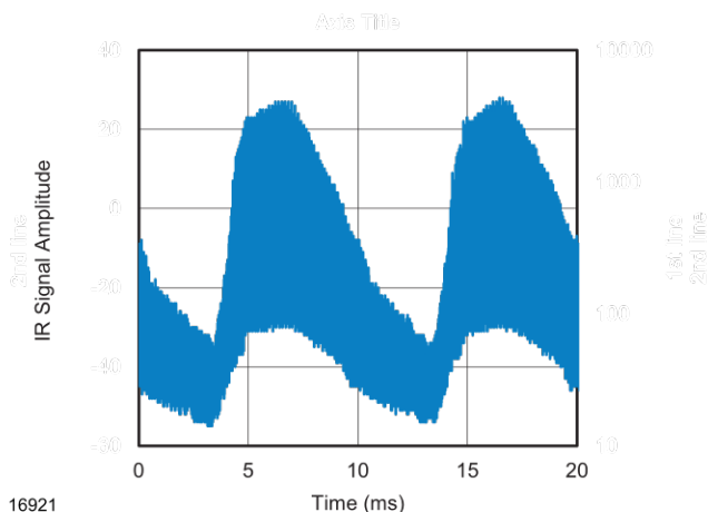
Fig. 14 - IR Disturbance from Fluorescent Lamp With High Modulation
