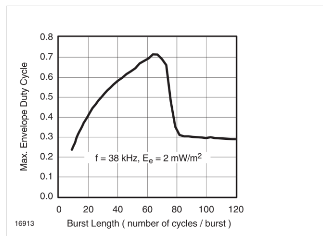
Figure 9. Max. Envelope Duty Cycle vs. Burstlength
