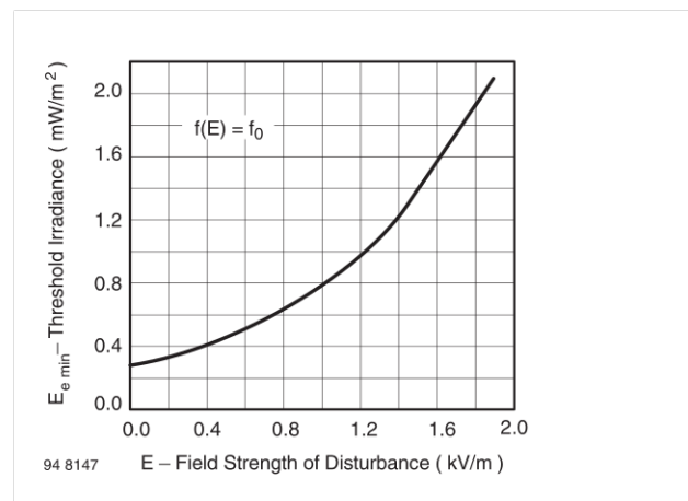
Figure 8. Sensitivity vs. Electric Field Disturbances
