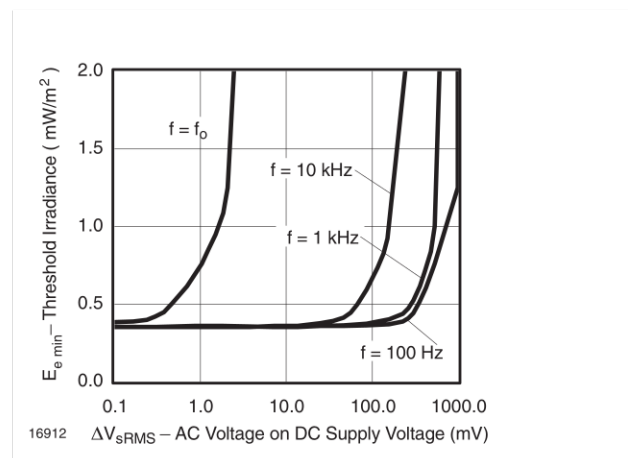
Figure 7. Sensitivity vs. Supply Voltage Disturbances
