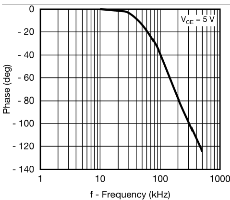
Fig. 12 - CTR Frequency vs. Phase Angle
