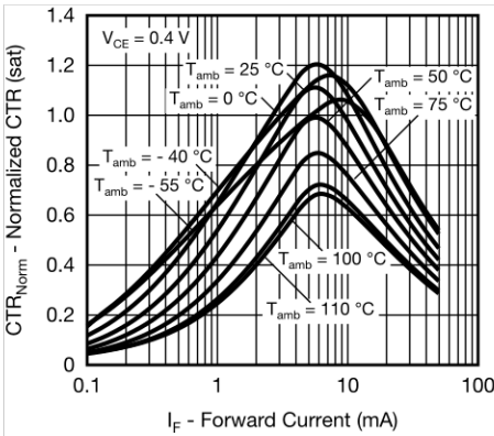
Fig. 11 - Normalized CTR (sat) vs. Forward Current
