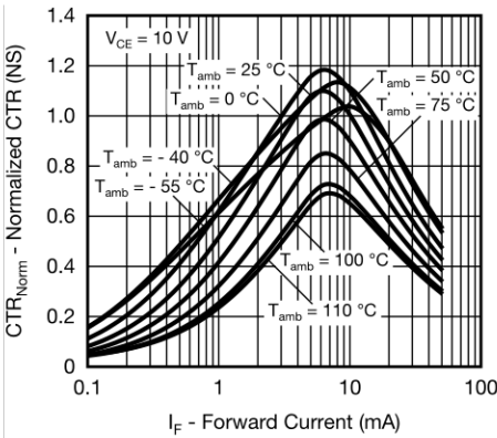
Fig. 10 - Normalized CTR (NS) vs. Forward Current
