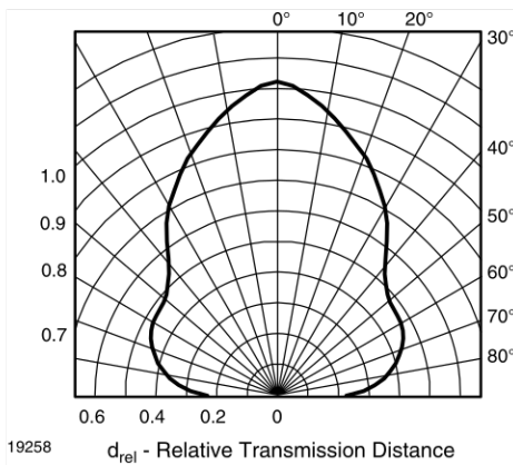
Fig. 11 - Horizontal Directivity
